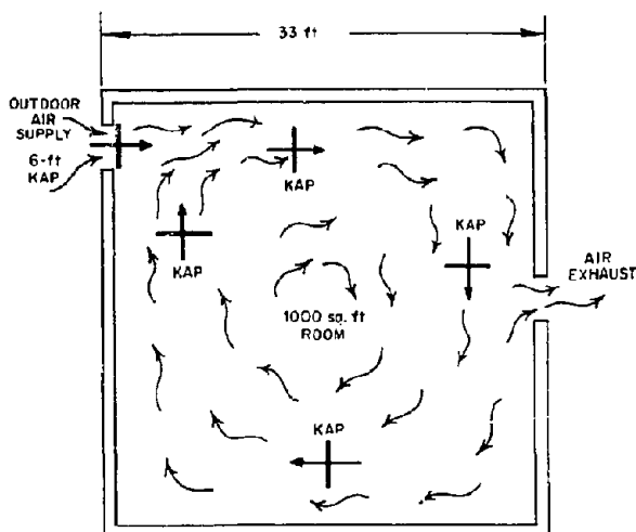
Fig. B-16. Air distribution in large shelter.
